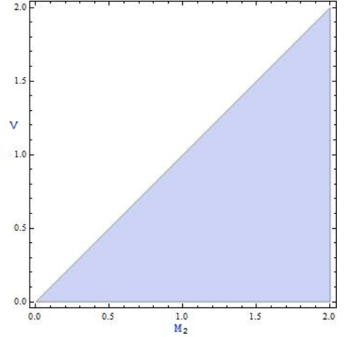
FIG. 3: The figure shows the amount of measurement dependence required on bob's side to simulate any nonlocal correlation for an one sided local deterministic model.
