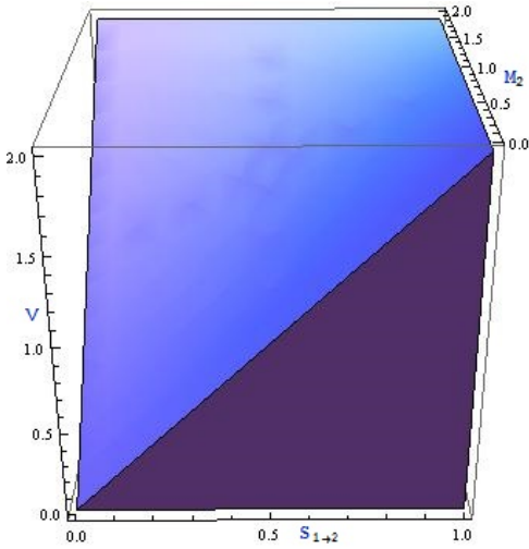
FIG. 2: The figure represents the tradeoff between signaling, indeterminism and the amount of violation for S_{1 \rightarrow 2} \geq 1 - 2I_2 . In particular, region lying on the V S_{1 \rightarrow 2} plane (i.e M_2 = 0 plane) represents the amount of signaling required for V amount of violation of Bell-CHSH inequality.
