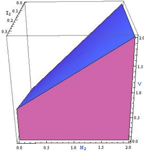
FIG. 4: For S_{1 \rightarrow 2} < 1 - 2I_2 case when I_2 = 1/3 then the minimum amount of measurement dependence required to simulate any amount of violation ( V ) is given by the I = \frac{1}{3} plane.
