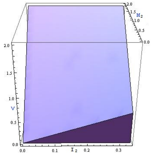
FIG. 1: The tradeoff between I_2 and M_2 for any amount of V is plotted when S_{1 \rightarrow 2} < 1 - 2I_2 . Clearly, the maximum value that the upper bound B(I_2, S_{1 \rightarrow 2}, 0) can achieve is 2.67 for S_{1 \rightarrow 2} < 1 - 2I_2 .
