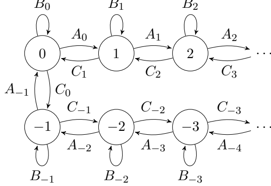
FIGURE 3. Folded walk of \Phi on \mathbb{Z}_{\geq 0} \times \{1, 2\} given by \check{\Phi} .
