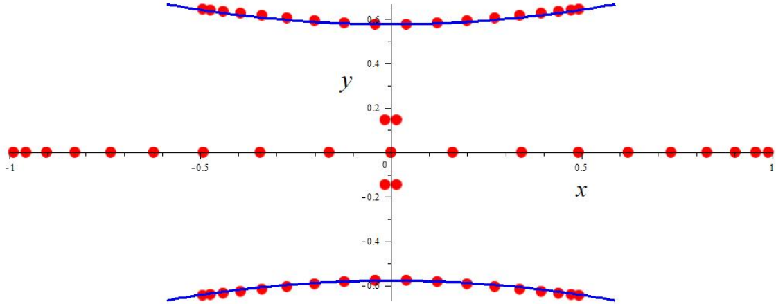
FIGURE 4. Eigenvalues of \check{\Phi} with 20 vertices.
