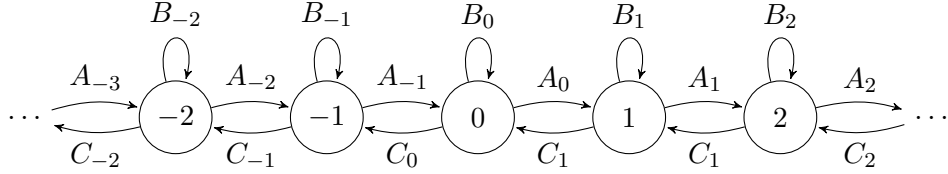
FIGURE 2. QMC \Phi on \mathbb{Z} .
