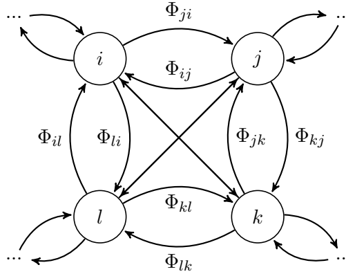
FIGURE 1. Schematic illustration of QMCs. The walk is realized on a graph with a set of vertices denoted by i, j, k, l, \dots and each operator \Phi_{ij} is a completely positive map describing a transformation in the internal degree of freedom of the particle during the transition from vertex j to vertex i . For simplicity of illustration some edges are not labeled. In the particular case that all maps are conjugations, i.e., for every i, j , \Phi_{ij} = B_{ij} \cdot B_{ij}^* for certain matrices B_{ij} the QMC is called an open quantum walk. In this work, the graphs considered will be either a line segment, the half-line, or the integer line.
