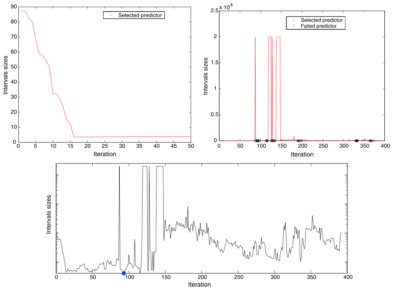
Fig. 2 (Color online) Analysis of conformal predictors length (y-axis) through the LASSO modification of the LARS algorithm iterations (x-axis: the first iteration corresponds to \lambda_{\max} and the last one corresponds to \lambda_{\min} ) in Example (c)[300/1] (top left) and in Example (c)[50/1] (top right). The iteration associated to the CoLP is
