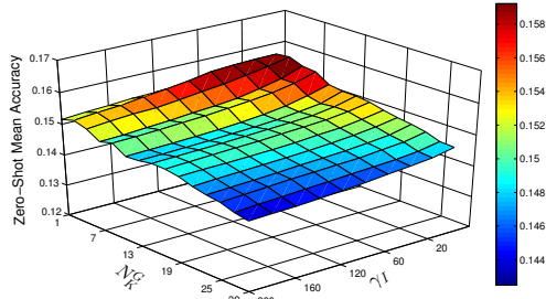
(a) HMDB51
