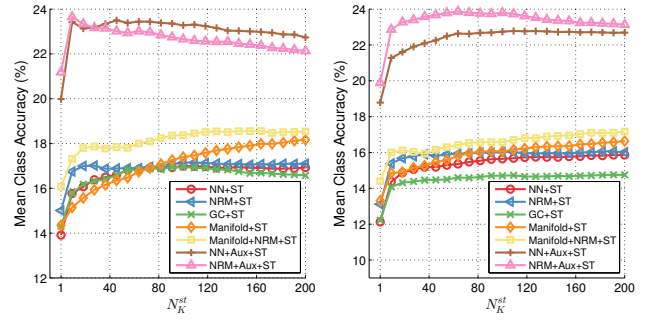
(a) HMDB51
