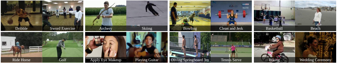
(a) HMDB51
