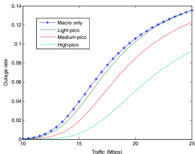
Fig. 4 Cell outage rate ( P_{\text{pico}}=30 W)
