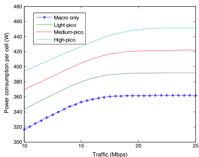
Fig. 5 Power consumption in the cell ( P_{\text{pico}}=30 W)
