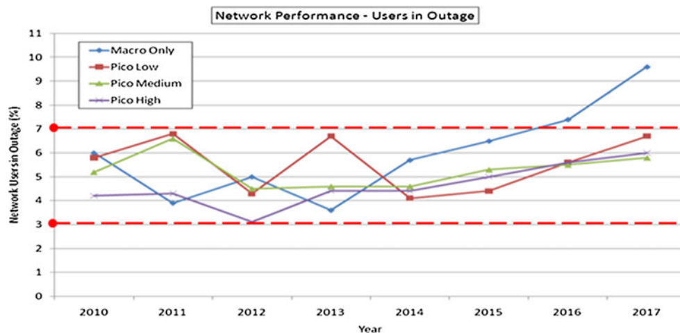
Fig. 12 Network performance in terms of percentage of users in outage, highlighting the target acceptable areas
