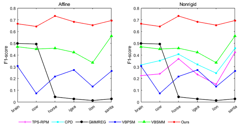
Fig. 8 The average F1-scores after applying six methods on six shapes under the affine (left) and nonrigid (right) cases with random degrees of rotation and outliers
