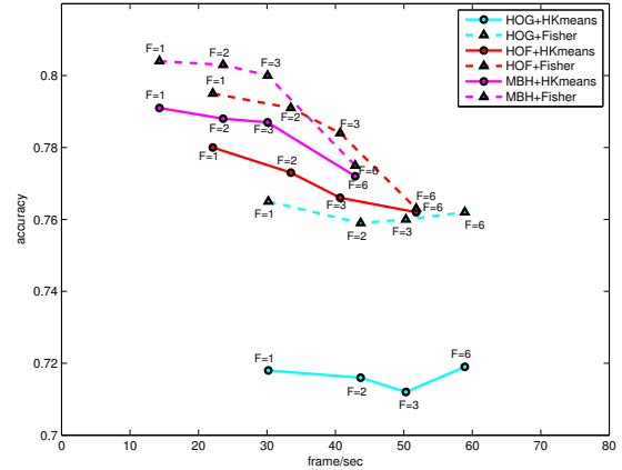
Fig. 6: Trade-off accuracy/efficiency when varying sampling rate. F stands for frames per block and it is directly related to sampling rate.
