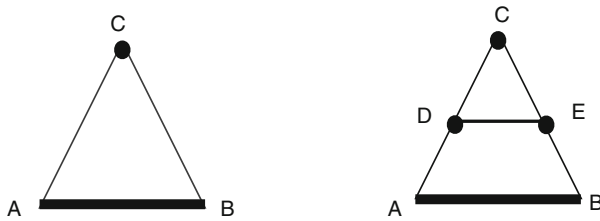
Fig. 1 The 2-simplex K and its subcomplex L = [A, B] \cup \{C\} on the left; a subdivision of the complement K - L producing an induced subcomplex on the right (it is obtained in two step, firstly by adding the vertex D and secondly by adding E )
