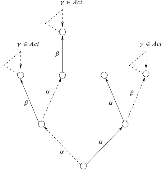
Fig. 7. The operational meaning of the term \alpha_{\perp} . (\beta_{\sharp} . \perp + \alpha_{\perp} . \beta_{\sharp} . \perp) + \alpha_{\sharp} . (\alpha_{\sharp} . \mathbf{0} + \beta_{\perp} . \perp) is a partial modal transition tree in that its leaves either deadlock ( \mathbf{0} ) or model a may-stub ( \perp ) that loops for all events \gamma \in Act
