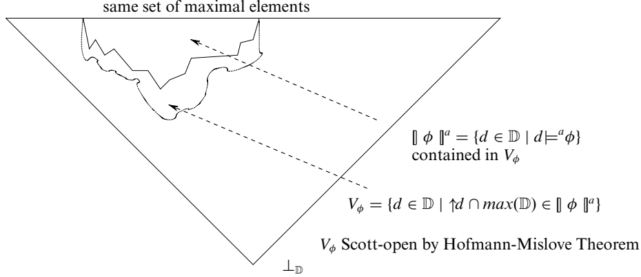
Fig. 12. A schematic description of the potential loss of precision of \equiv^a over \equiv^{a+} represented by V_\phi \setminus \llbracket \phi \rrbracket^a . The properties of \llbracket \phi \rrbracket^a and V_\phi stated in this figure are shown subsequently, except for V_\phi \cap \max(\mathbb{D}) = \llbracket \phi \rrbracket^a \cap \max(\mathbb{D}) which is obvious
