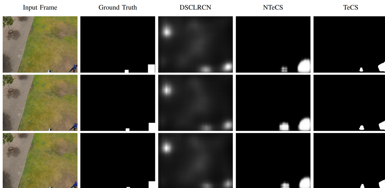
Fig. 2 Performance of models on the 'person9' sequence from UAV123 [6], used in our test set. Shown are three consecutive frames near the start of the sequence. Note: the ground truths have been modified for qualitative evaluation (see above discussion of the UAV123 dataset)
