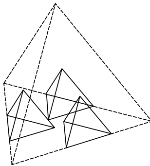
Figure 3: A counterexample in \mathbb{R}^3 for three tetrahedra
