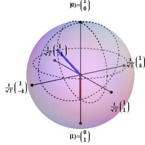
Fig. 1 The amplitude damping channel
