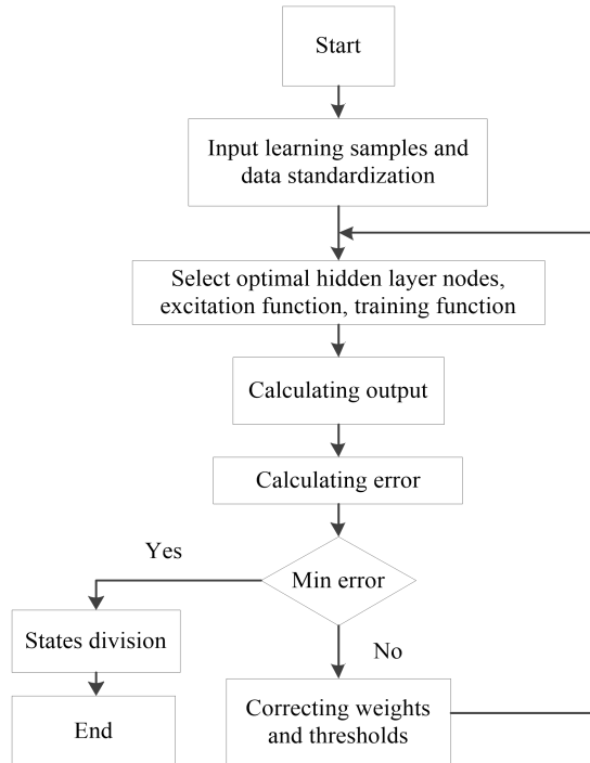
Figure. 4 The process of the BP algorithm.
