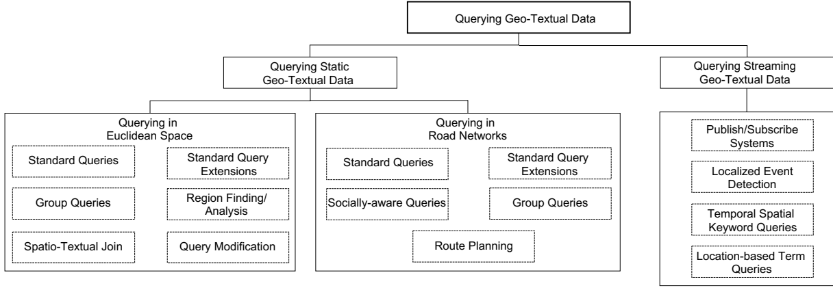
Fig. 2 Geo-Textual Query Classification Framework
