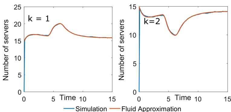
Fig. 3 Number of servers allocated to each queue over time—two classes with dynamic server allocation, parameters from Table 3
