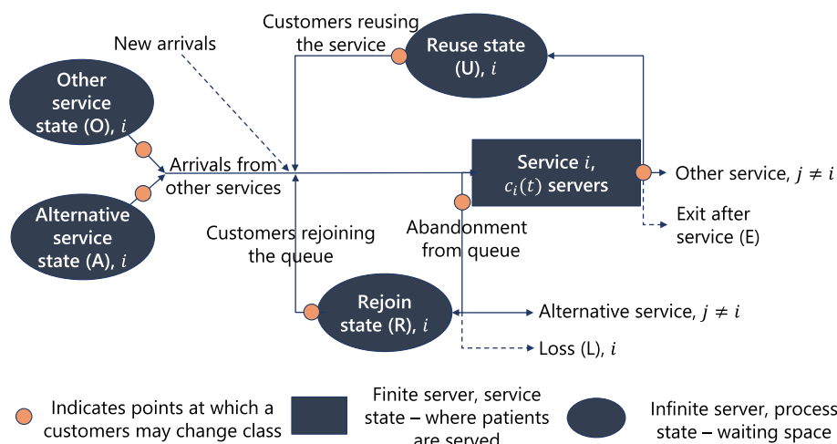
Fig. 1 Diagram of general customer flow in all classes through a single service within the stochastic queueing network
