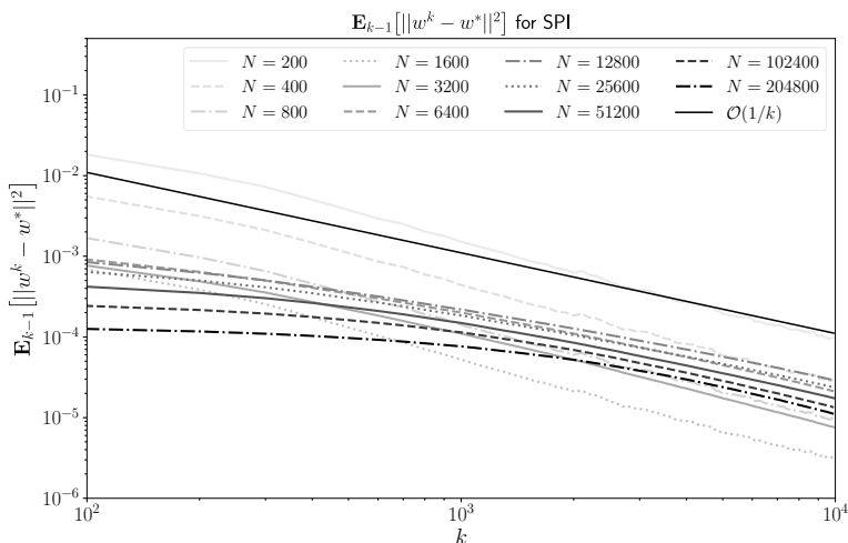
Fig. 1 Approximated errors \mathbf{E}_{k-1} [\|w^k - w^*\|_N^2] for the SPI method, measured in RMS-norm, for discretizations with varying number of grid points N . Statistics were only computed at every 100 time steps, this is why the plot starts at k = 100 . The 1/k -convergence is clearly seen by comparing to the uppermost solid black reference line
