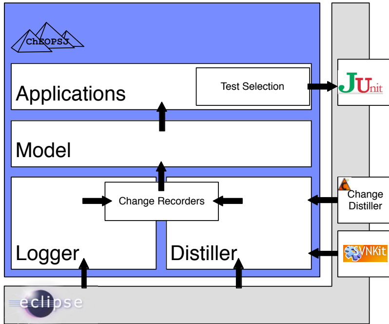
Fig. 5: The layered design of ChEOPSJ.
