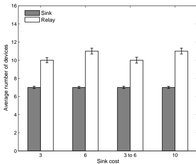
Fig. 14 Average numbers of sinks and relays for CBS-MSRP with MaxIter = 200 versus sink cost
