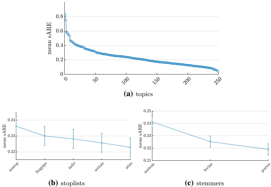
Fig. 9 Main effects for topics, stoplists and stemmers of sMARE-AP from MD0_{micro} for the QPP models on the Robust04 title queries. We also report the confidence interval for stoplists and stemmers. We do not report CI for the topics, for the sake of image readability (Color figure online)
