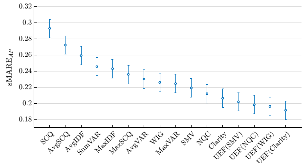
Fig. 8 Confidence Intervals of sMARE-AP from MD0_{micro} for the QPP models on the Robust04 title queries (Color figure online)
