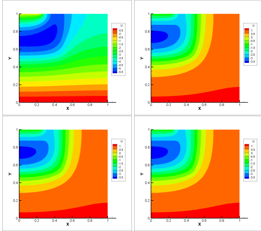
Figure 2: From left to right, from top to bottom are the contour plots of \phi_h at time: T = 0.01, 0.4, 0.7, 1 for Example 2.
