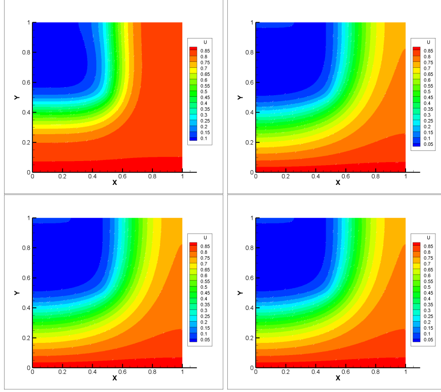
Figure 1: From left to right, from top to bottom are the contour plots of u_h at time: T = 0.01, 0.4, 0.7, 1 for Example 2.
