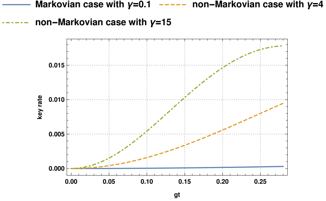
FIG. 3: (Color online) Plot of secure key rate with respect to the dimensionless time gt , for the Case 2, where the both travel and home qubits are subject to NMAD noise. Here \gamma is the coupling strength and g := 1 in all the cases. In the considered time range, non-Markovian noise provides improvement in the key rate as seen for the cases of \gamma = 4 (dashed, orange curve) and \gamma = 15 (dot-dashed, green curve), as opposed to the Markovian case with \gamma = 0.1 (bold, blue curve).
