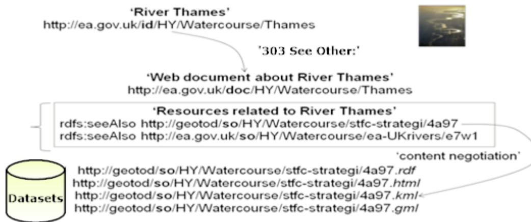
Figure 8: Use of HTTP URIs and RDF vocabulary to identify, expose and link related Web-based resources.
