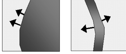
Figure 4. The two configurations favoured by the quadratic image term.
