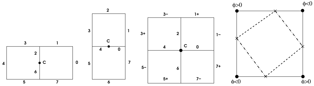
Figure 3. Leftmost three: configurations encountered in the contour tracing algorithm. Right: an ambiguous configuration.
