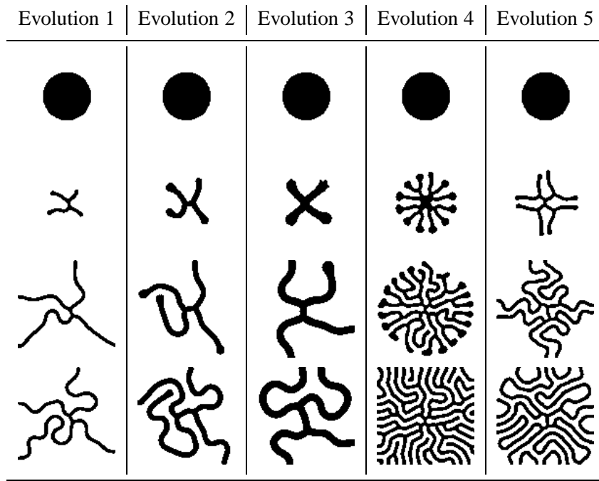
Figure 2. Examples of gradient descent using the energy in equation (11). The first three columns correspond to different values of d_{\min} , while the last two correspond to different values of \alpha .
