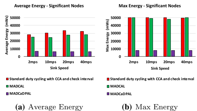
Fig. 19 Average and maximum energy consumption of significant nodes (mWs). Transmission range 62.02m, Random topology. MADCaDPAL
