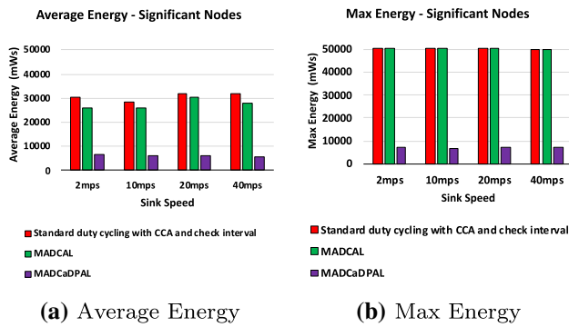
Fig. 20 Average and maximum energy consumption of significant nodes (mWs). Transmission range 55.94m, Random topology. MADCaDPAL
