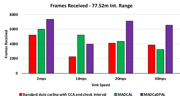
Fig. 13 Sink frame reception. Transmission range 77.52m, Grid topology. MADCaDPAL
