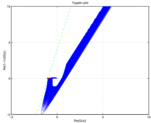
Figure 7 Set of Tsykin plots which all satisfy the frequency condition (17) for G_z = G_z(K, T_i) , where (K, T_i) correspond to pole locations to the left upper stability triangle A_1 in Figure 6.
