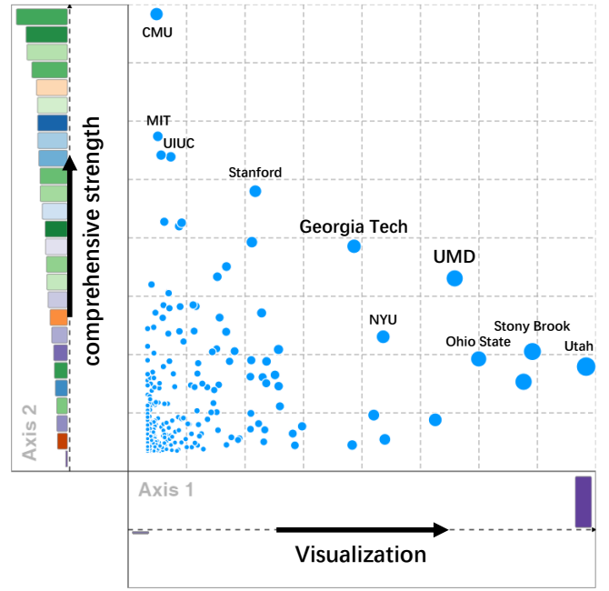
Fig. 7. A simple example of a composite custom semantic space. The distribution of institutions (points) indicates that the correlation between the performance in the VIS and the comprehensive strength is small. Georgia Tech and College Park are among the few options for institutions that have achieved great rankings in both aspects.
