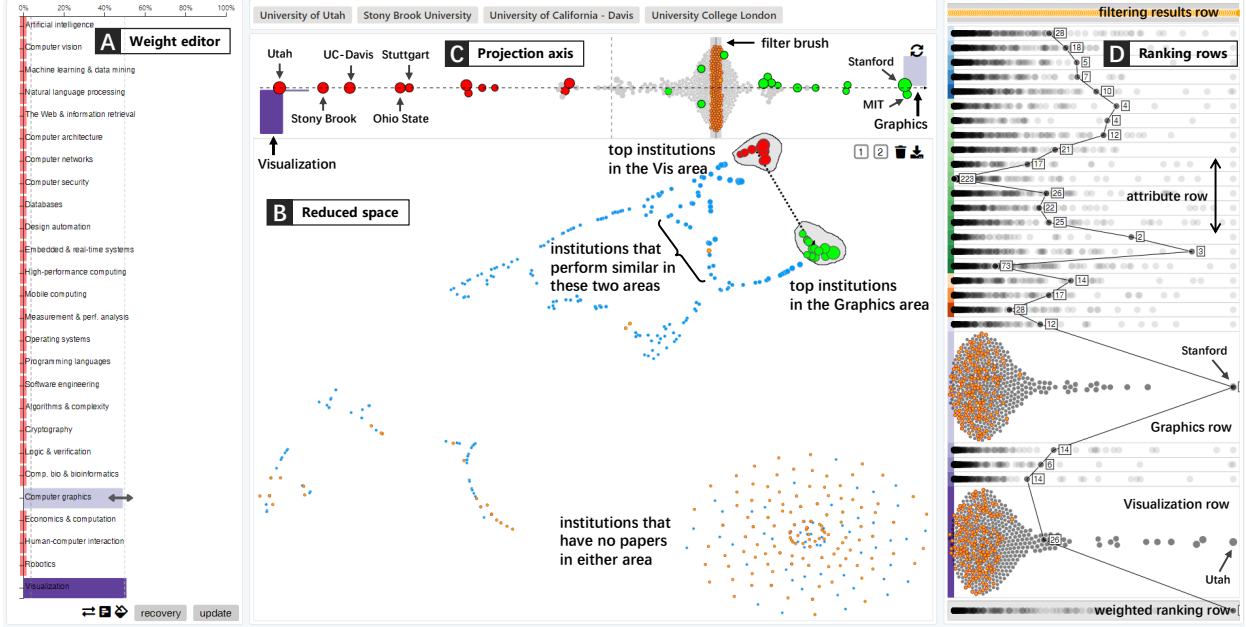
Fig. 1. Interface of our system. With weight editor, analysts are free to emphasis or ignore attributes by adjusting their weights (the light red rectangle reminds the analyst that the weight of the corresponding attribute has been or will soon be reduced to zero). Reduced space presents dimension reduction results and allows analysts to construct SemanticAxis by lassoing two groups of points. Projection axis is designed for interpreting a constructed axis and checking its semantics distribution in reduced space. Ranking rows are used to verify inferences by providing details of data points (space for those emphasised attributes is expanded to enable individual checking).
