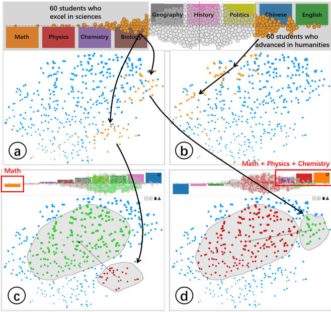
Fig. 9. Biased students found by SemanticAxis are distributed on the lower right (a), partial to the sciences) and upper left (b, partial to humanities) sides of the reduced space. The differences between the two groups of students in (a) lay in that the former only excel in math (c) while the latter is good at math, physics, and chemistry (d).
