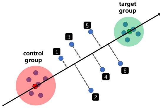
Fig. 2. Illustration for SemanticAxis. SemanticAxis is a vector that passes through the center of two groups of high-dimensional data selected by the analyst. It serves as a metric for the semantic strength of data points whose rankings according to their projected position on the axis.
