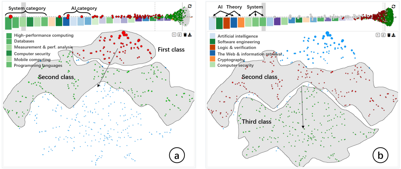
Fig. 11. Institutions in upper class perform better than those in lower class in all areas. Nevertheless, the differences between the first (top 80) and second class (81th ~ top 50%) are significantly different from that between the second and third class (last 50%). It is mainly reflected in the conspicuous forward movement of areas under AI and Theory category in the later.
