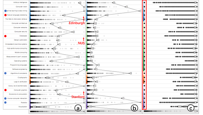
Fig. 4. Illustration of the three scale strategies in attribute rows: scale with values of individual attribute, values of all attributes, and rankings. (a) demonstrates that, for most areas of computer science (especially for the areas labeled with red node), there are a handful of institutions that perform noticeably well. (b) shows that, the scale of the top conferences of blue-node areas is much larger than that of other areas. The large blank on the left of (c) indicates that, for all areas, there are a significant number of institutions (in the red box) failed to publish in the corresponding top conferences.
