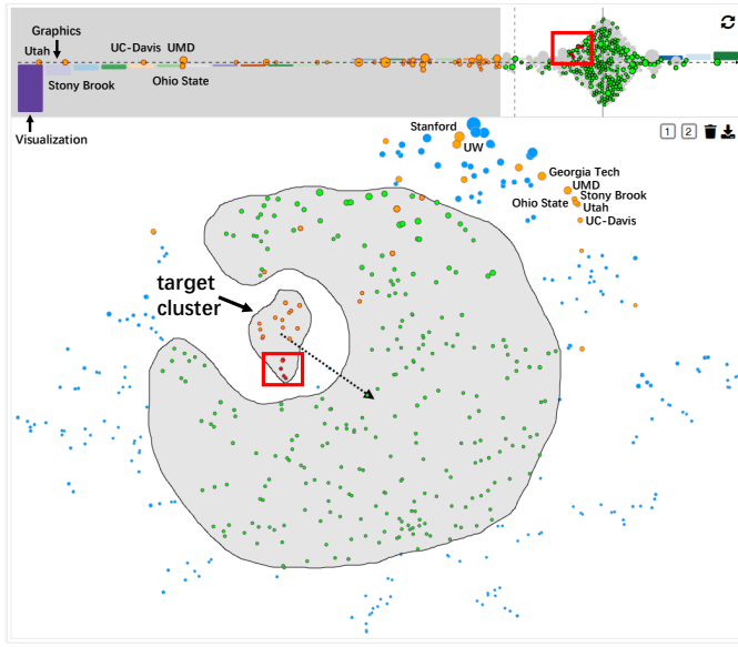
Fig. 12. Insights uncovered by checking the lassoed cluster: four institutions (shown in the red box) should not have been selected; the exact semantics of the focused cluster is that it includes institutions that are nearly only excellent in the VIS area.
