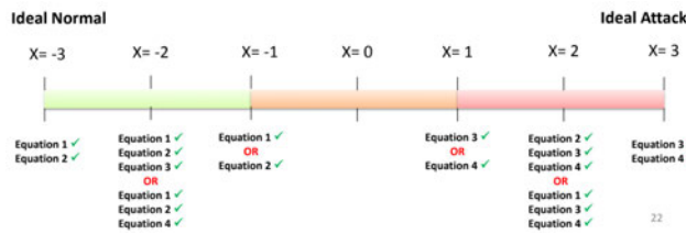
Fig. 2 The relevancy of network packet counts and their ratio to the Attack/Normal states (used in Sign 2)
