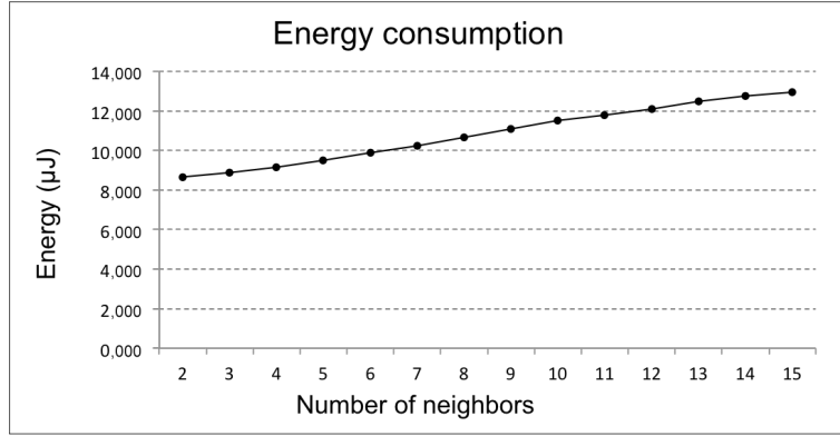
Figure 11: Energy consumption of a boundary node S_1 .
