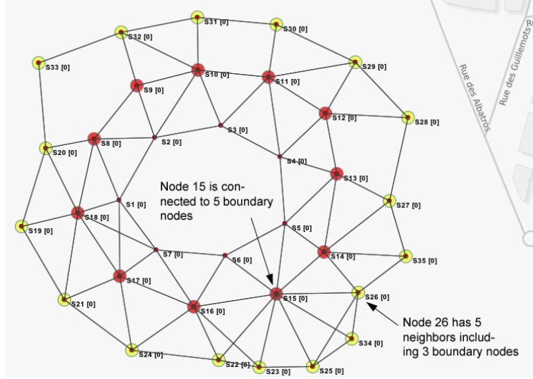
Figure 13: A Wireless Sensor Network with 35 nodes.
