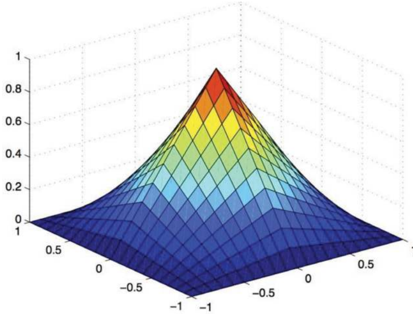
Figure 1. The exact Fourier transform in Example 2.
