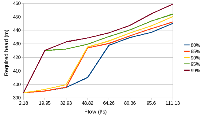
Figure 5: Pump profiling in the "Boutre" network.
