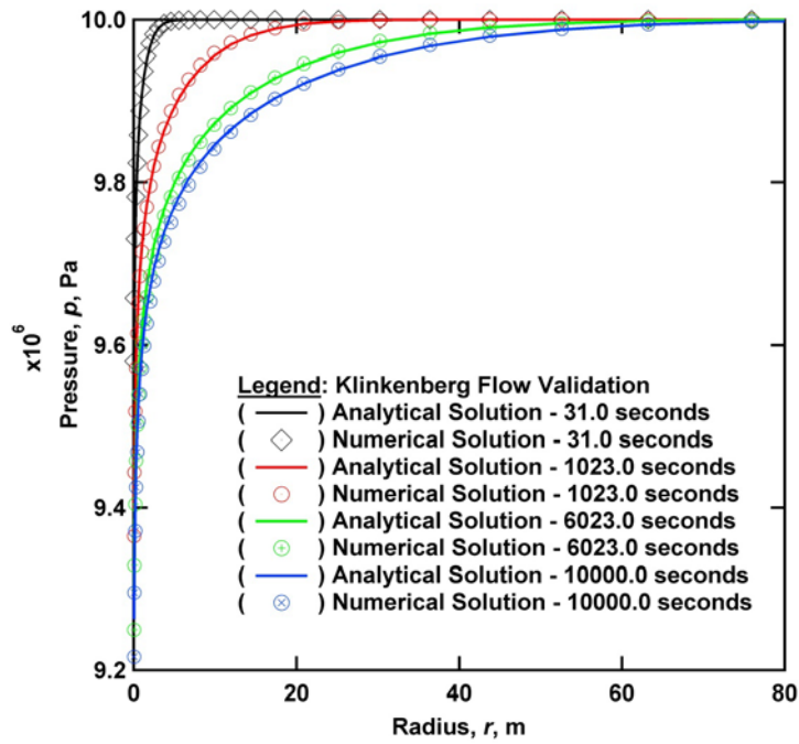
Figure 5 — Validation of the T+G code against the analytical solution of Wu et al. (1988) in Problem V4 of Klinkenberg flow in a cylindrical gas reservoir. The T+G and T+GW solutions are identical.
