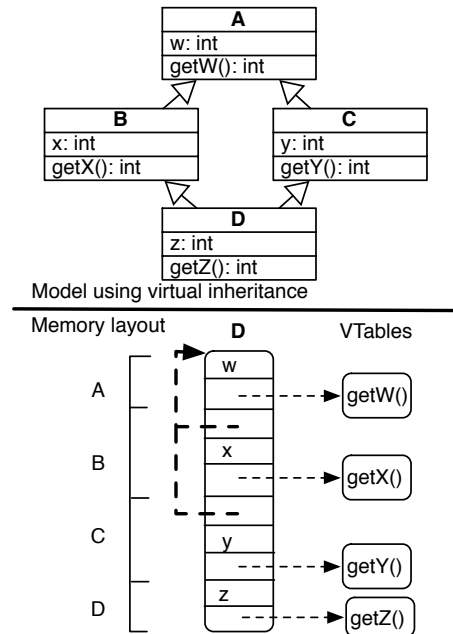
Fig. 21. Multiple virtual inheritance in C++.
