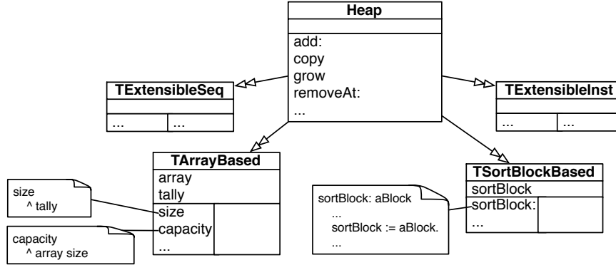
Fig. 25. Refactoring of the class Heap with stateful traits removing the trait THeapImpl .
