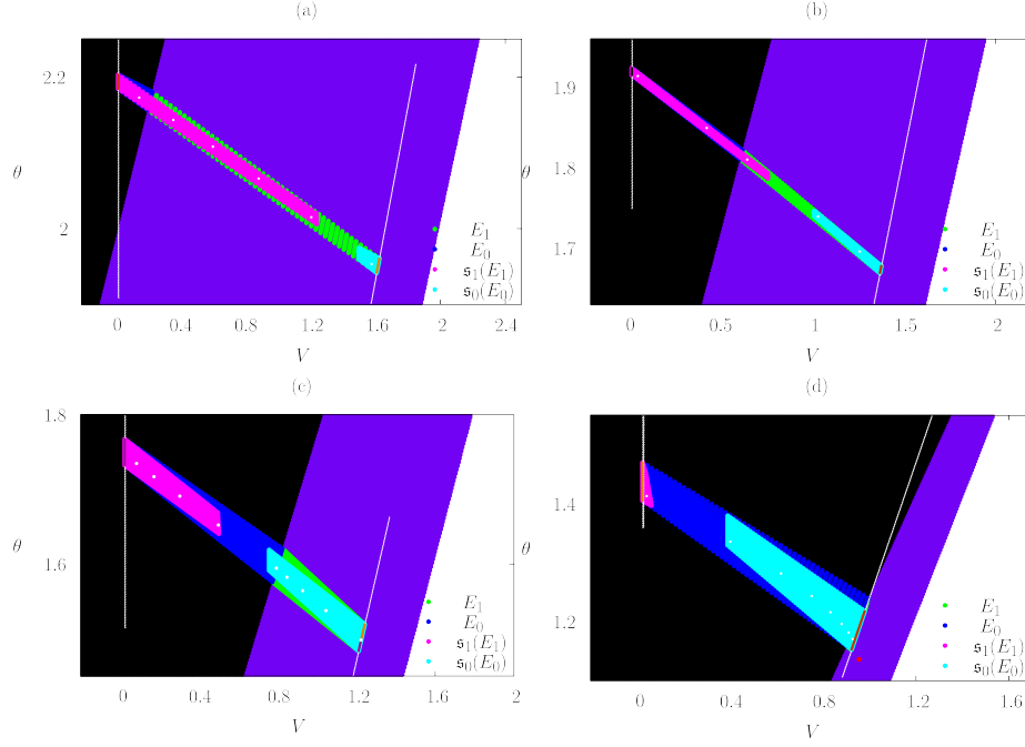
Figure 14: Sets E_i satisfying condition i ) of Theorem 1 for the parameter values labeled in Figure 11(a). The found periodic orbits have symbolic itineraries: (a) 01^5 , (b) 0101^2 , (c) 0^21(01)^3 and (d) 0^71 . The corresponding evolution of V and \theta with respect to time is shown in Figure 13. White points are the periodic orbit found by direct simulation. Red point is a virtual fixed point found by extending the maps \mathfrak{s}_i in their virtual domains, as explained in Section 3.2. Black background is S_0 , blue background is S_1 . Blue and green sets are E_0 and E_1 , respectively. Pink and light blue are \mathfrak{s}_1(E_1) and \mathfrak{s}_0(E_0) , respectively. The white lines are the images \mathfrak{s}_0(\Sigma_1) and \mathfrak{s}_1(\Sigma_1) . Colored lines are the images of \gamma (see text) by \mathfrak{s}_i . Those segments that stay connected for all iterates of \mathfrak{s} are plotted with the same color. For Figure (c), not all iterates of the \Sigma_1 stay connected and, hence, does not satisfy condition iii). For (c) and (d) we have found points in E_1 whose differential D\mathfrak{s}_1 has eigenvalues outside the unit circle, and hence condition ii) is not satisfied. (a) and (b) satisfy conditions i )– iii ) of Theorem 1.
