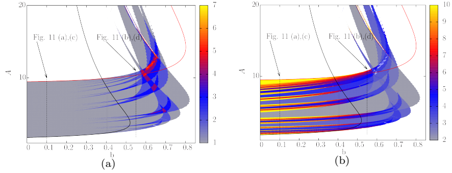
Figure 10: (a) Number and (b) period of the periodic orbits of the stroboscopic map for T = 0.5 stepping on S_0 and S_1 found by means of the numerical algorithm described in Appendix D. We include also the bifurcation curves computed in Figure 4. All periodic orbits are maximin. The areas where there is coexistence of two or more periodic orbits are colored according to an averaged period in order to reflect superposition of colors. Regions with orbits of period equal or higher than 10 have the same color. Notice that the region where periodic orbits exist shows a jagged edge due to numerical issues related to grazing of the orbits.
