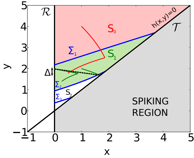
Figure 1: Trajectories of system (22)-(24) with initial conditions in sets S_0 (red) and S_1 (green), plotted on top of the pieces S_0 , S_1 , S_2 where the stroboscopic map is defined. Boundaries \Sigma_1 , \Sigma_2 and \Sigma_3 are computed using the algorithm described in Appendix A. Solid black curves correspond to the threshold manifold \mathcal{T} and the reset manifold \mathcal{R} . Parameter values for the system are c = 0.53 , V_0 = 0.1 , A = 2 , \tau = 2 , T = 3 , \Delta = 0.3 and b = 0.1 .
