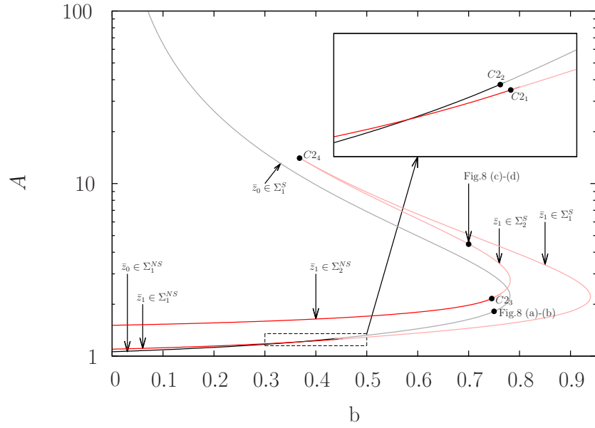
Figure 7: Border collision bifurcation curves and regions of existence of the fixed points \bar{z}_0 and \bar{z}_1 in the (b, A) parameter space for T = 5 (vertical axis in logarithmic scale). Curves in black and gray correspond to border collision bifurcations of \bar{z}_0 \in S_0 with \Sigma_1^{NS} and \Sigma_1^S , respectively. Curves in red and light red correspond to border collision bifurcations of \bar{z}_1 \in S_1 with \Sigma_2^{NS} and \Sigma_1^S , respectively. Co-dimension-two bifurcation points are labeled as C2_i , i = 2, 3, 4 and are explained in the text. Dots on these curves indicate the parameter values (A, b) for which we show (in the Figure indicated nearby) the trajectory of the periodic orbit of the time continuous system that undergoes a grazing bifurcation.
