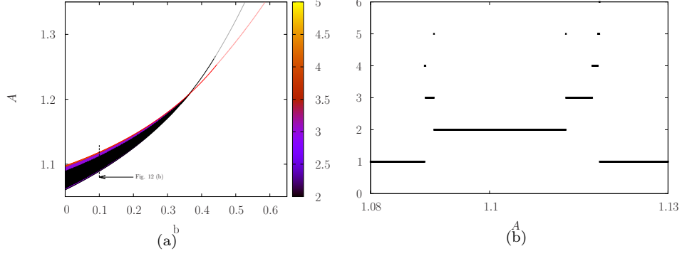
Figure 12: (a) Periods of unique maximin periodic orbits of the stroboscopic map for T = 5 stepping on S_0 and S_1 . We include also the bifurcation curves computed in Figure 7. (b) Periods of the periodic orbits found by varying the amplitude A along the vertical line b = 0.1 as indicated in panel (a).
