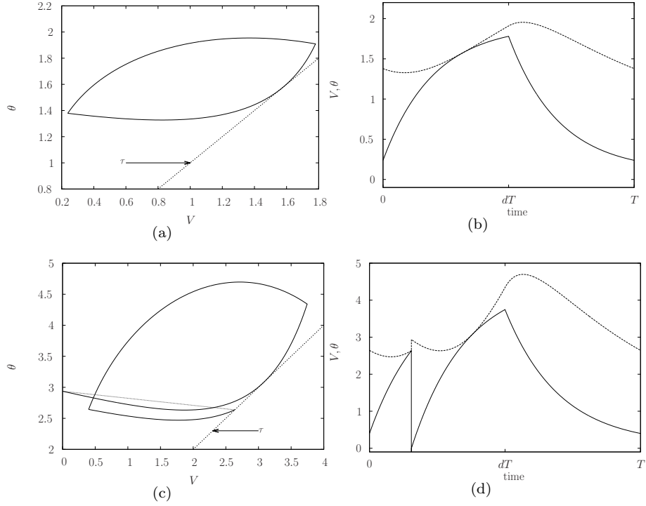
Figure 8: Trajectories of T -periodic orbits undergoing the smooth grazing bifurcations labeled in Figure 7. (a)-(b) Smooth grazing bifurcation of a non-spiking periodic orbit (border collision of \bar{z}_0 \in S_0 with \Sigma_1^S ). (c)-(d) Smooth grazing bifurcation of 1-spiking periodic orbit (border collision of \bar{z}_1 \in S_1 with \Sigma_2^S ).
