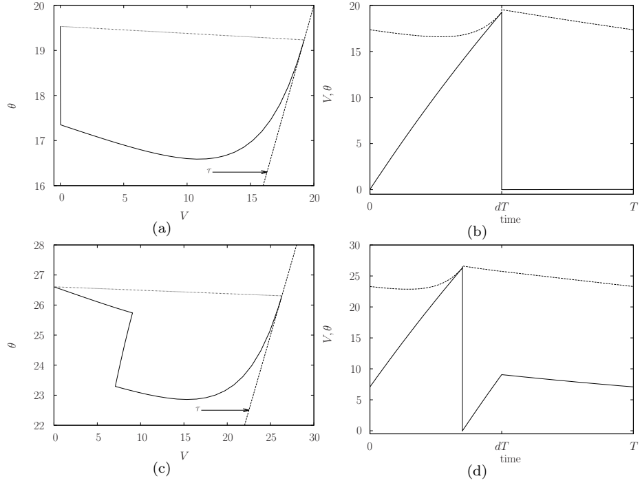
Figure 6: Trajectories of T -periodic orbits undergoing the grazing bifurcations labeled in Figure 4. (a)-(b) Co-dimension two bifurcation labeled as C2_1 in Figure 4; a periodic orbit undergoes a smooth bifurcation at t = dT ( \bar{z}_1 \in S_1 collides with \Sigma_1^{\text{NS}} and \Sigma_1^{\text{S}} simultaneously). (c)-(d) Smooth grazing bifurcation of a 1-spiking periodic orbit (border collision of \bar{z}_1 \in S_1 with \Sigma_1^{\text{S}} .) Left panels show trajectories on the (V, \theta) -phase space while right panels show the corresponding time courses of the variables V (solid line) and \theta (dashed line) over 1 period.
