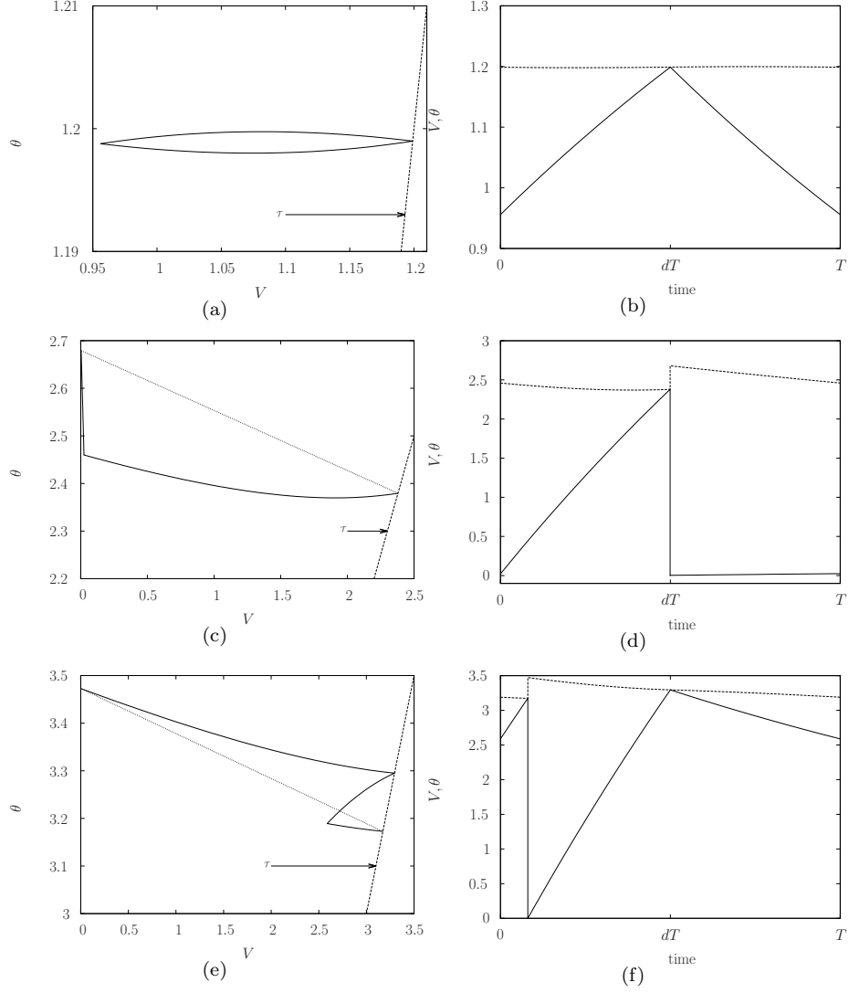
Figure 5: Trajectories of T -periodic orbits undergoing the grazing bifurcations labeled in Figure 4. (a)-(b) Nonsmooth grazing bifurcation of a non-spiking periodic orbit (border collision of \bar{z}_0 \in S_0 with \Sigma_1^{\text{NS}} ). (c)-(d) Nonsmooth grazing bifurcation of a 1-spiking periodic orbit (border collision of \bar{z}_1 \in S_1 with \Sigma_1^{\text{NS}} ). (e)-(f) Nonsmooth grazing bifurcation of a 1-spiking periodic orbit (border collision of \bar{z}_1 \in S_1 with \Sigma_2^{\text{NS}} ). Left panels show trajectories on the (V, \theta) -phase space while right panels show the corresponding time courses of the variables V (solid line) and \theta (dashed line) over 1 period.
