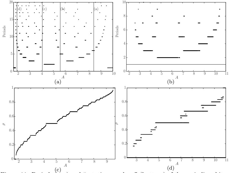
Figure 11: Periods (top) and “rotation numbers” (bottom) of the periodic orbits found by varying the amplitude A along the vertical lines b = 0.1 (left) and b = 0.55 (right) as indicated in Figure 4. Periodic orbits have been computed numerically using the algorithm described in Appendix D. For b = 0.1 , we repeated the computations with a smaller stepsize along the A -axis and we have found higher periods interleaved according to the Farey tree structure (results not shown), suggesting that the “rotation number” shown in (c) might be continuous along the Farey tree.
