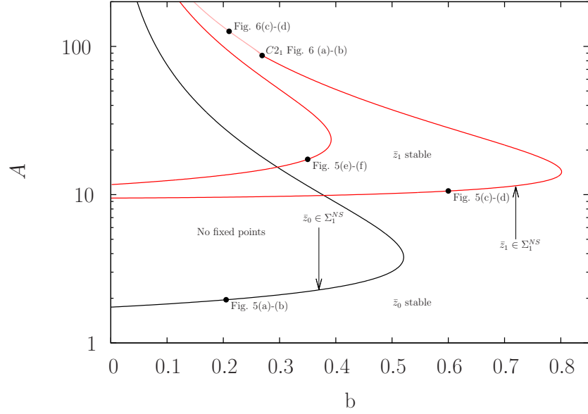
Figure 4: Border collision bifurcation curves and regions of existence of \bar{z}_0 and \bar{z}_1 in the (b, A) parameter space for T = 0.5 (vertical axis is in logarithmic scale). Curve in black corresponds to a border collision of \bar{z}_0 \in S_0 with \Sigma_1^{NS} . Curve in dark red corresponds to a border collision of \bar{z}_1 \in S_1 with \Sigma_1^{NS} (outer curve) and \Sigma_2^{NS} (inner curve). Curve in light red corresponds to a border collision of \bar{z}_1 \in S_1 with \Sigma_1^S . Dots on these curves indicate the parameter values (A, b) for which we show (in the Figure indicated nearby) the trajectory of the periodic orbit of the time continuous system that undergoes a grazing bifurcation.
