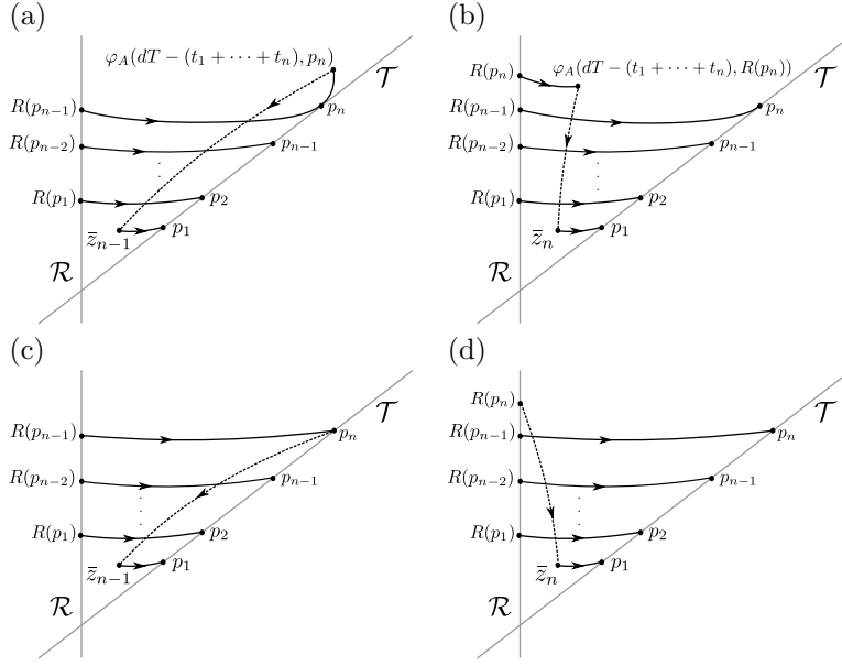
Figure 2: Scheme showing a periodic orbit of the system (1)-(3) (a,b) grazing tangentially the manifold \mathcal{T} at the point p_n and (c,d) grazing the manifold \mathcal{T} at the non-differentiable point p_n at time dT . These periodic orbits correspond to fixed points of the stroboscopic map hitting the manifold \Sigma_n^S (a,b) and the manifold \Sigma_n^{NS} (c,d). Panels (a,c) correspond to a collision of a point \bar{z}_{n-1} \in S_{n-1} with \Sigma_n , while panels (b,d) correspond to a collision of the point \bar{z}_n \in S_n with \Sigma_n . See Section 4 for more details. Solid black lines correspond to trajectories of the flow \varphi_A , while dashed black lines correspond to trajectories of the flow \varphi_0 . Grey lines correspond to the reset manifold \mathcal{R} and the threshold manifold \mathcal{T} .
