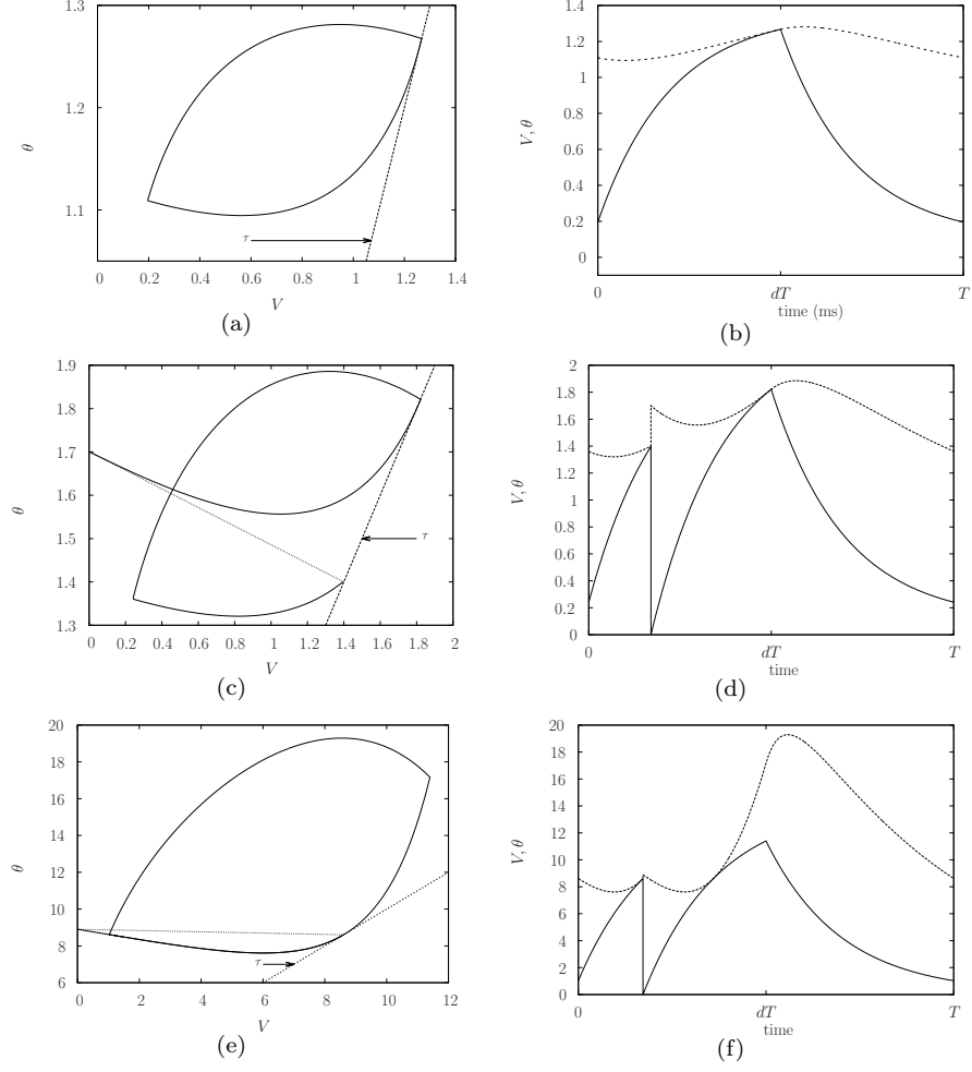
Figure 9: Trajectories of the T -periodic orbits at the co-dimension two bifurcation points labeled in Figure 7. (a)-(b) Point C2_2 : a non-spiking periodic orbit tangentially grazes the threshold at t = dT ( \bar{z}_0 \in \Sigma_1^{\text{NS}} \cap \Sigma_1^{\text{S}} ). (c)-(d) Point C2_3 : a 1-spiking periodic orbit tangentially grazes the threshold precisely at t = dT , when the pulse is disabled ( \bar{z}_1 \in \Sigma_2^{\text{NS}} \cap \Sigma_2^{\text{S}} ). (e)-(f) Point C2_4 : a 1-spiking periodic orbit grazes the threshold twice, both tangentially ( \bar{z}_1 \in \Sigma_1^{\text{S}} \cap \Sigma_2^{\text{S}} ).
