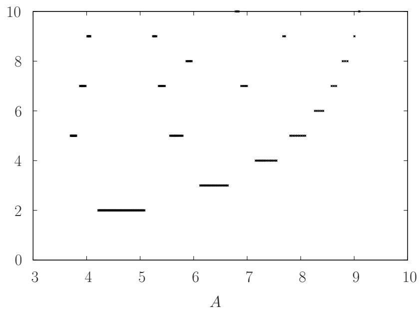
Figure 15: Periods of the periodic orbits in Figure 11(a) satisfying conditions of Theorem 1.
