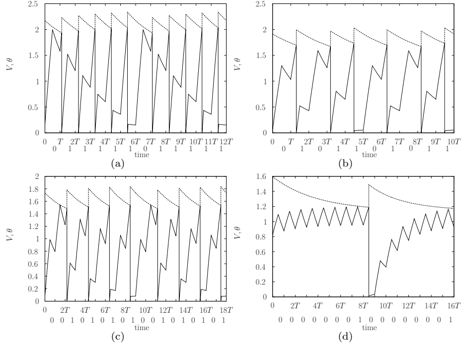
Figure 13: Time course of the variables V (solid) and \theta (dashed) corresponding to the four nT -periodic orbits labeled in Figure 11(a) (with n = 6, 5, 9 and 8 for panels (a), (b), (c) and (d), respectively). Notice that we show two periods of the nT -periodic orbits. We indicate their symbolic itinerary at the bottom of the time axis.
