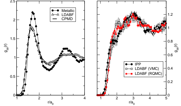
Fig. 6. Left panel: r_s = 1 , T = 1500K , N_p = 54 . Proton-proton pair correlation functions as obtained with LDABF and metallic wave functions. Results are obtained with TABC by using twist sampling around a 4 \times 4 \times 4 grid. CPMD data from ref.[15] are also represented by a thick dashed line. Right panel: r_s = 1.4 , T = 2000K , N_p = 54 . Proton-proton pair correlation functions as obtained with IPP and LDABF wave functions. Results are obtained with TABC by using a 6 \times 6 \times 6 fixed grid (IPP) and by twist sampling around a 4 \times 4 \times 4 grid (LDABF).
