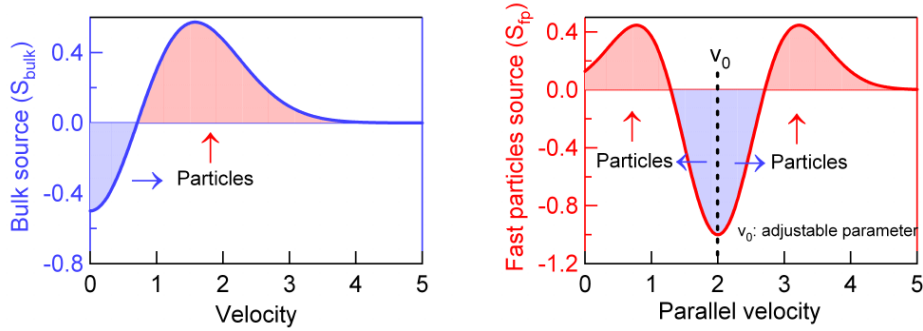
Figure 2: Schematic view of the energetic particle source as a function of the parallel velocity
