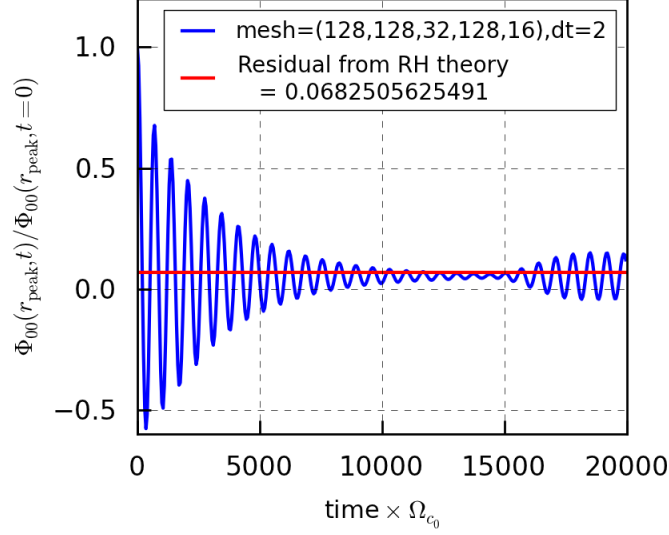
Figure 9: Comparison of the residual value of the (0,0) mode \phi_{00}(r_{\text{peak}}, t) / \phi_{00}(r_{\text{peak}}, t = 0) = A_r where A_r = 1/(1 + 1.6q^2/\sqrt{r/R}) = 0.06825 is given by Rosenbluth-Hinton theory. This result corresponds to simulation 1 described in Table 8.
