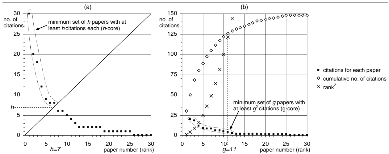
Fig. 2 – Graphical representation of (a) the h -index and (b) the g -index. Graphs are constructed using the input data reported in Fig. 3.
