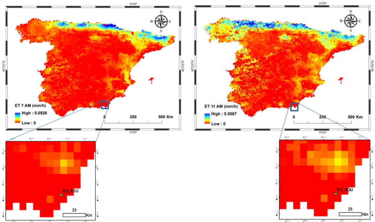
Figure 7: Maps of the SEVIRI ET final pre-processed product using our SEVIRI Pre-Pro software here for August 6 th , 2011 acquired at 2 different times of the day (7 am pm left and 11am right) for the ES_AGU site in Spain in the zoomed area.
