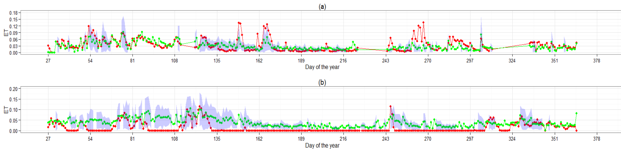
Figure 8: A comparison between in-situ and predicted ET from SEVIRI for the different seasons for ES_AGU site years 2010 (top) and 2011 (bottom). Green represents the in-situ ET daily mean, Red is the SEVIRI-predicted ET, Blue is daily standard deviation of the in-situ ET.
