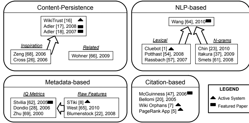
Figure 11: Relationships among publications (Wikipedia-centric)
