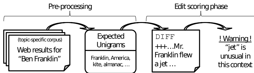
Figure 6: NLP - Example of semantic analysis
