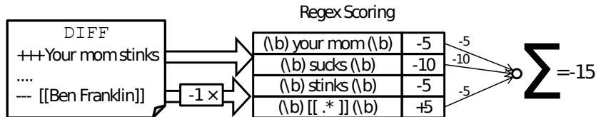
Figure 5: NLP - Example of lexical analysis
