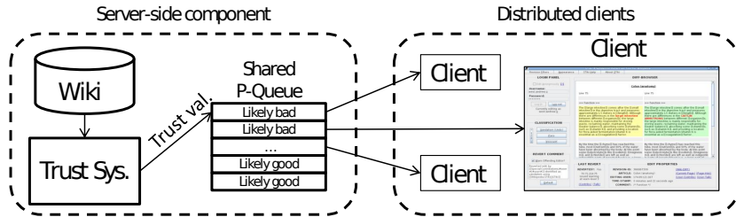
Figure 9: Example intelligent routing tool (STiki [8])
