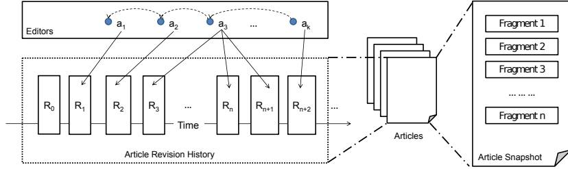
Figure 3: Relationships between wiki entities
