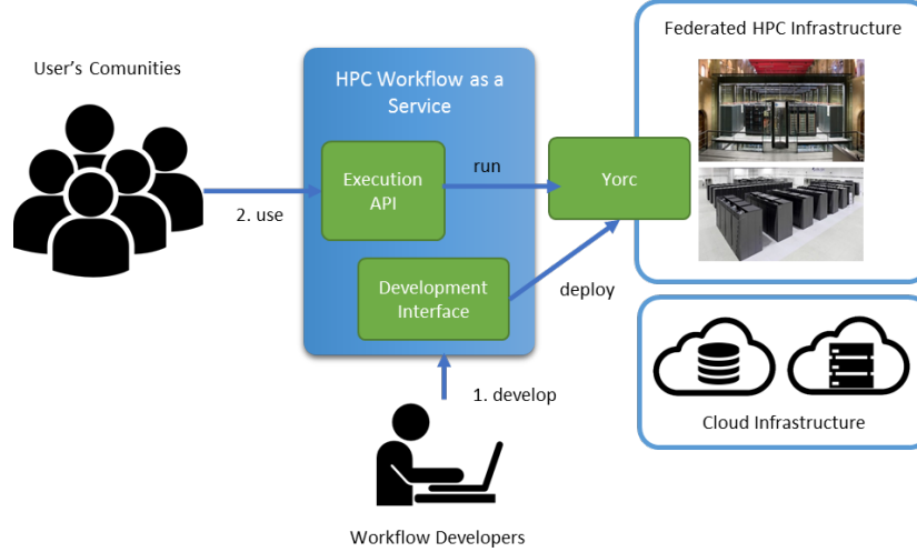
Figure 6: Overview of the proposed HPC Workflow-as-a-Service model.
