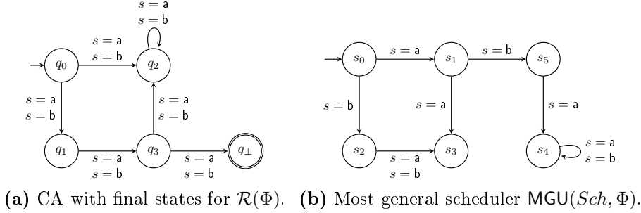
Figure 9: CAs of Example 8
