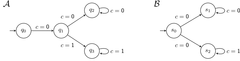
Figure 11: An example where tf_{\mathcal{A} \mapsto \mathcal{B}} is not the optimal transfer function.
