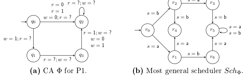
Figure 4: CAs of Example 4
