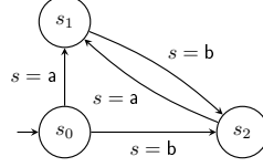
Figure 3: Most general scheduler Sch_v of Example 3
