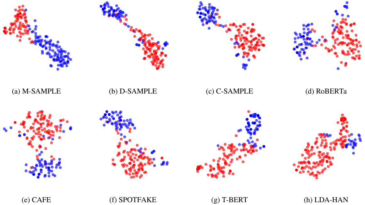
Figure 6: T-SNE visualizations of features learned before classifier from M-SAMPLE, D-SAMPLE, C-SAMPLE, RoBERTa, CAFE, SPOTFAKE, T-BERT and LDA-HAN on the test set of PoliFact in the 2-shot setting.
