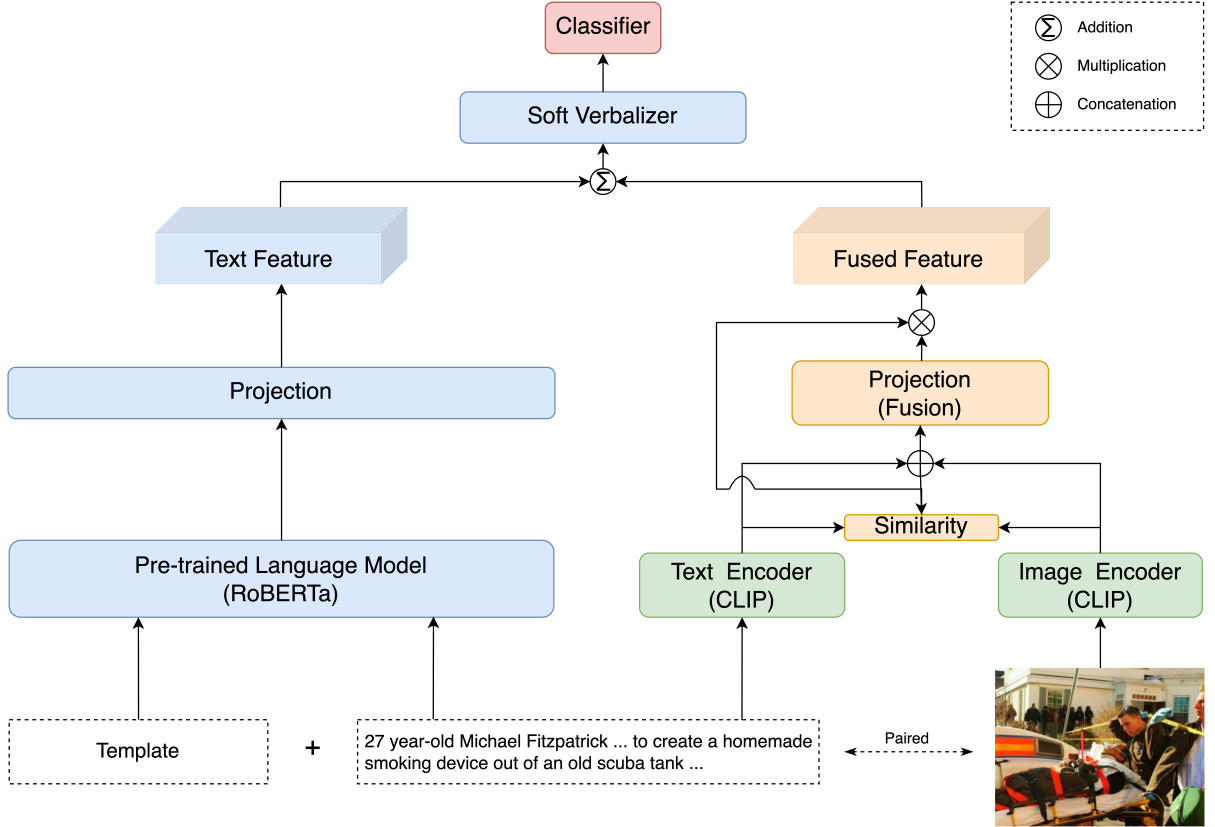
Figure 2: The overall structure of SAMPLE for fake news detection.
