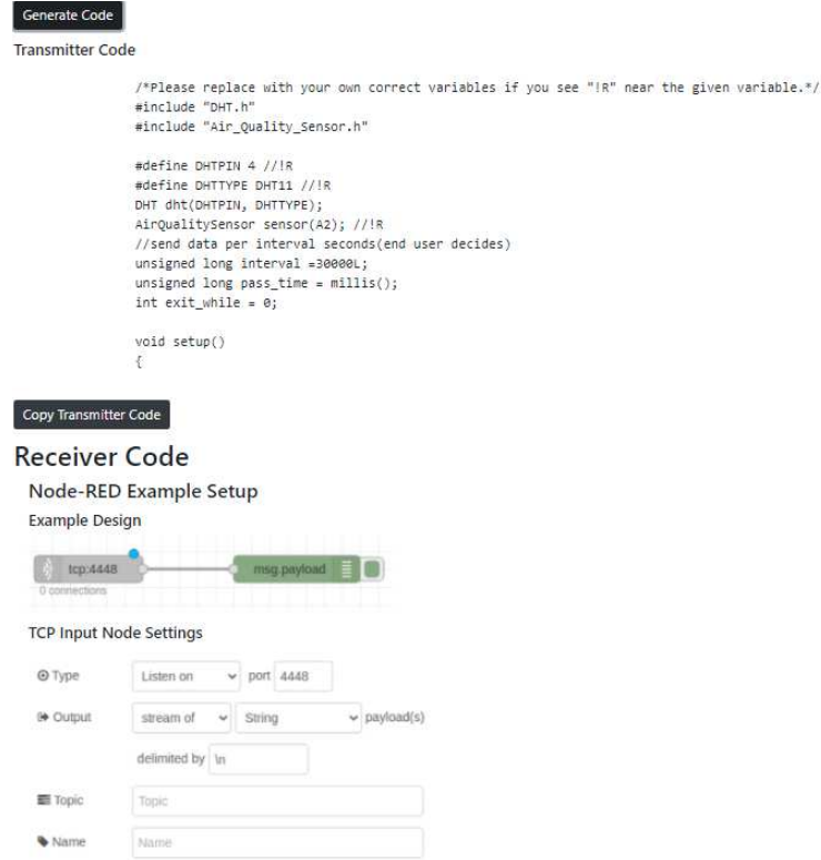
Figure 4: Illustrates the generated code block and the example Node-RED setup. In the example scenario, Raspberry Pi Pico is selected as an edge node/transmitter. The generated transmitter code is written in C++ and should be deployed via Arduino IDE. The Raspberry Pi 4B is acting as a fog node/receiver.
