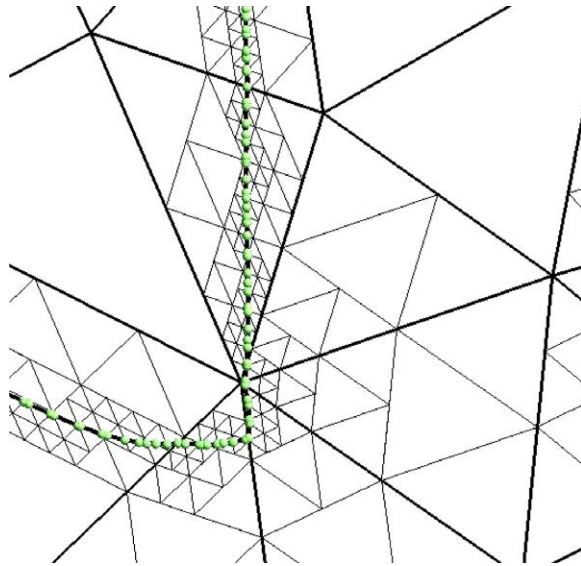
Fig. 4. Contouring algorithm to accurately localize the interface. In black, the computational mesh. In grey, the 4 level refined elements. In green, a set of points on the interface. (For interpretation of the references in colour in this figure legend, the reader is referred to the Web version of this article.)
