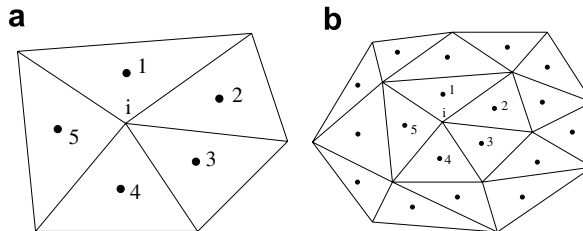
Fig. 6. Stencil used for the reconstruction of the gradient at node i . (a) Distance-1 stencil for the linear reconstruction (left), and (b) distance-2 stencil for the quadratic reconstruction (right).
