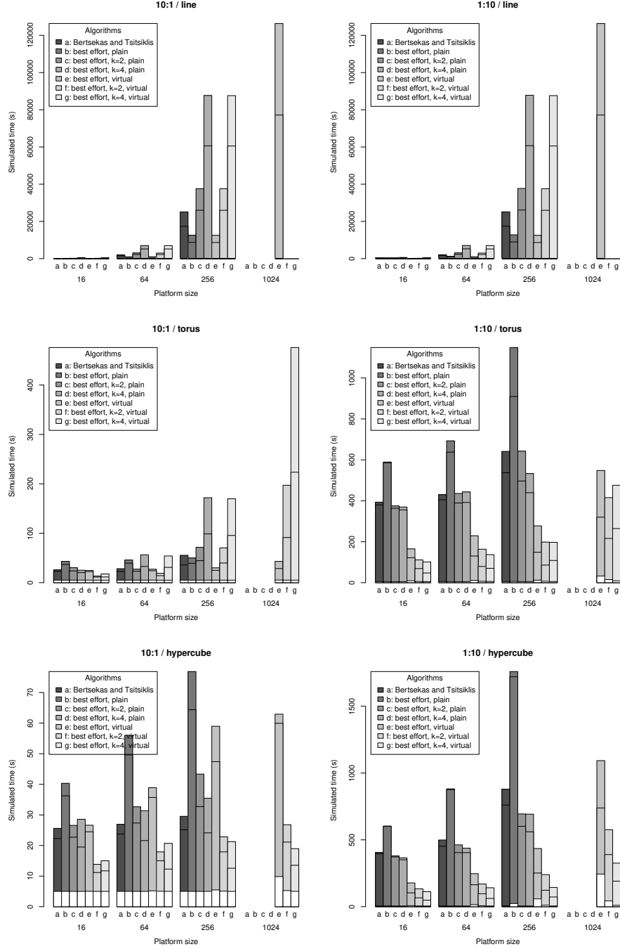
Figure 2: Real mode, random initial distribution, CCR = 10/1 (left), or 1/10 (right).
