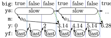
Fig. 14. “slow_fast” Async flow.
