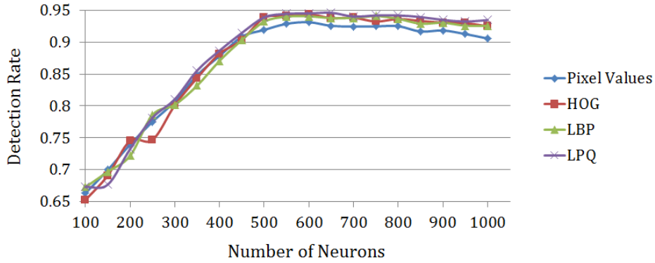
Figure 14. Detection rate VS number of neurons for the MIX database.
