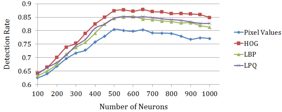
Figure 15. Detection rate VS number of neurons for the GENKI4K database.
