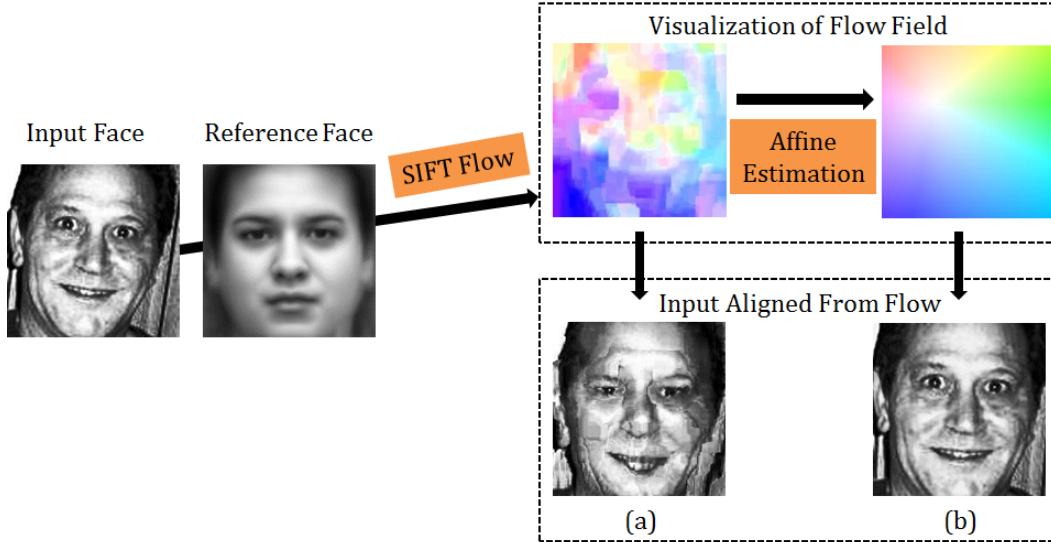
Figure 4. SIFT flow based face registration. The SIFT flow is first computed between the input face and the reference face. Affine estimation is used to transform the original discontinuous flow vector field to a smooth flow vector field. The aligned face using smoothed flow vector field contains much less artifact compared to the aligned face using the original flow vector field.
