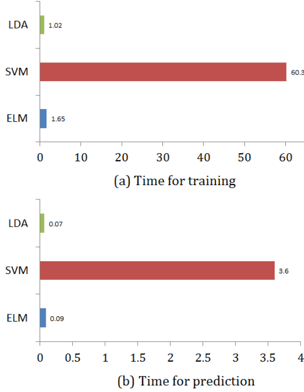
Figure 13. Computational cost for the GENKI4K database. (a) Training time (in s ). (b) Prediction time for one face (in ms ).
