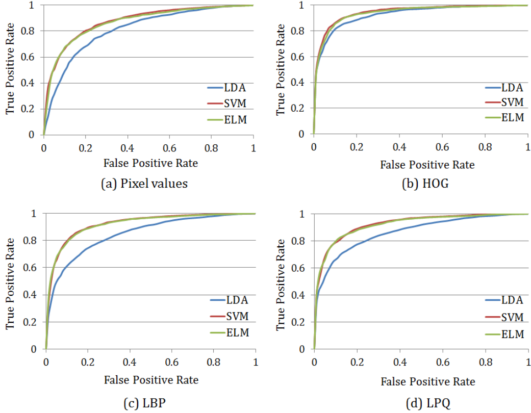
Figure 11. The ROC curves for the GENKI4K database with different feature descriptors. (a) Pixel values. (b) HOG. (c) LBP. (d) LPQ.
