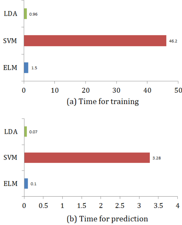
Figure 12. Computational cost for the MIX database. (a) Training time (in s ). (b) Prediction time for one face (in ms ).
