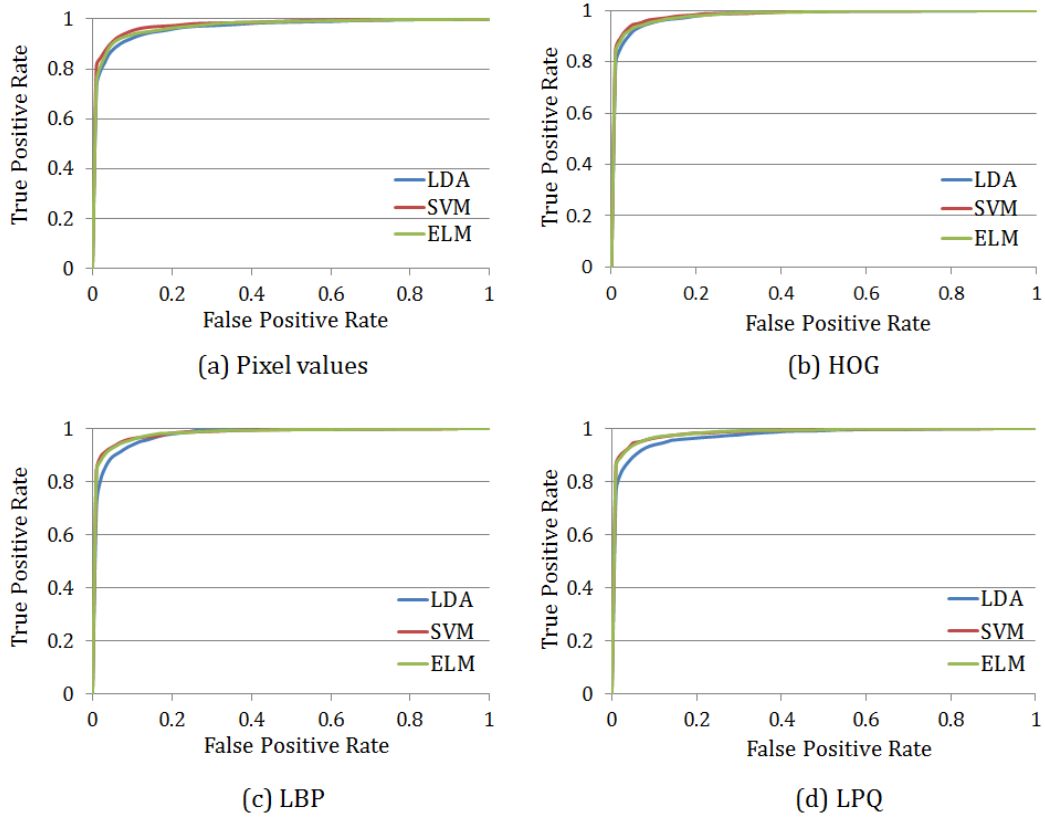
Figure 10. The ROC curves for the MIX database with different feature descriptors. (a) Pixel values. (b) HOG. (c) LBP. (d) LPQ.
