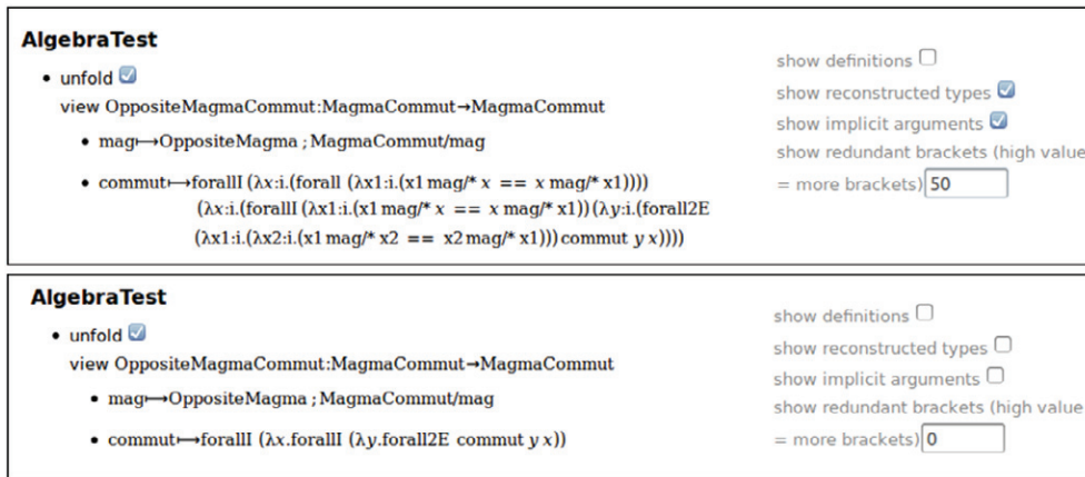
Figure 3: Formal Representations Adapted to Distinct User Settings (Customized via the DocDash Widget on the Right)
