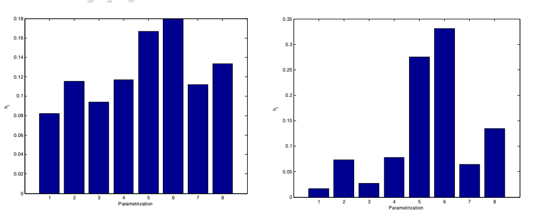
Figure 7 values of the h_j for different values of the Delta weight: 1 (left), 10 (right).
