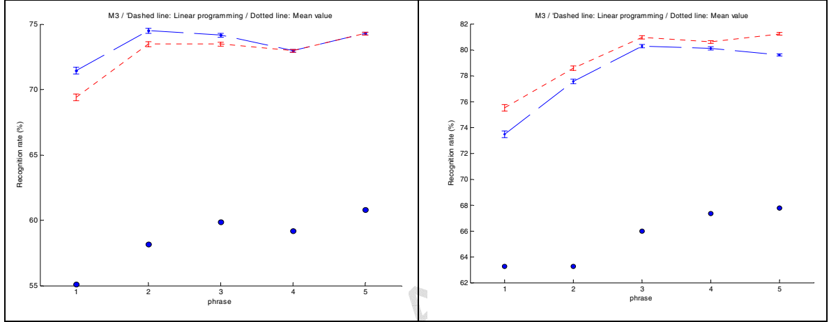
Figure 8 , Robustness of the method with respect to a change in the date of the recording. Setting M3 for Delta weights: 1 (left), 10 (right). Lower dots, correspond to the results of the MFCC alone.
