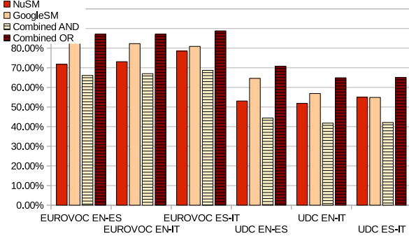
Combined F-measure.
