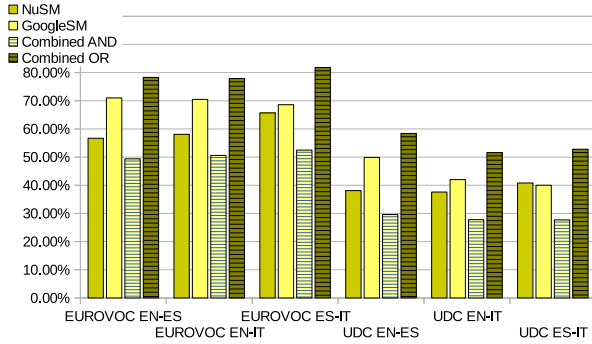
Combined recall.
