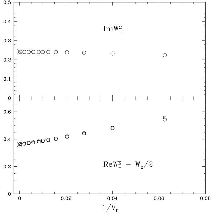
Fig. 2. The effective actions \text{Re} W_-^\Sigma - W_0/2 and \text{Im} W_-^\Sigma ( \circ ) for a pure toron field configuration with (t, \phi) = (0.5, \pi/8) and (e_\alpha, \epsilon_\alpha) = (1, -1) plotted against 1/V_f . Also shown is (1/2)W_V ( \square ). The numerical results are compared to the analytic results ( \times ) given in (2.28), (2.30).
